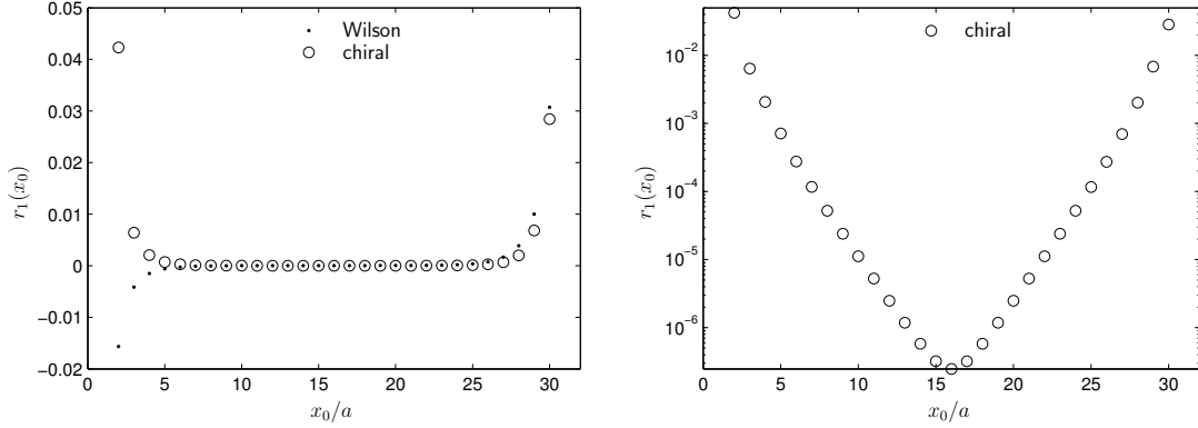
Figure 1: Bare current mass at 1-loop in PT (left). Logarithmic plot of this quantity for chiral fermions (right). The plots are for a 16 \times 32 lattice, \theta = 0 , N = 2 and g_V^2 = 0 .
