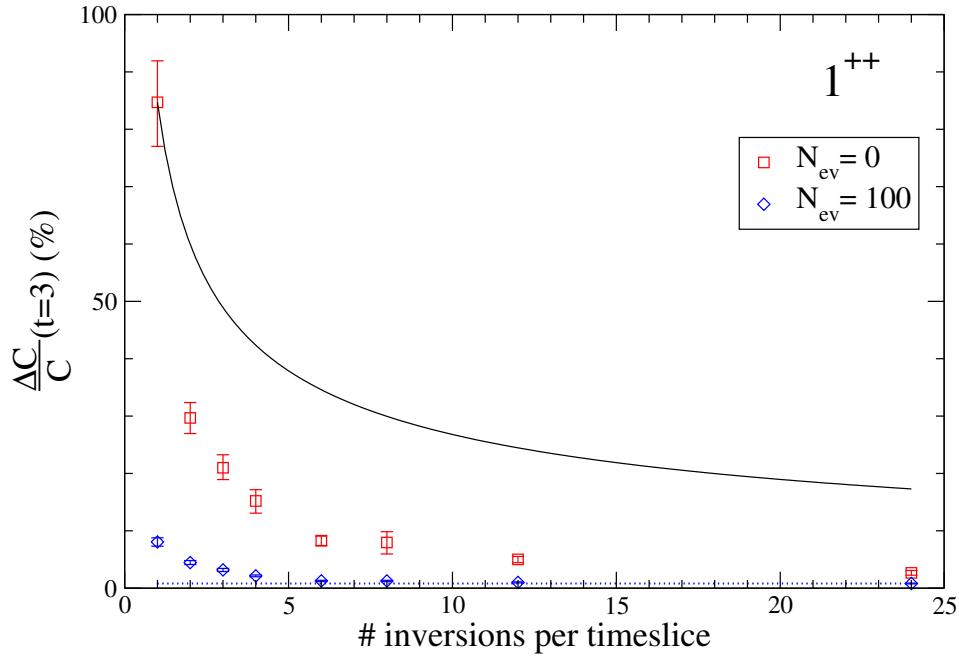
Fig. 9. As Fig. 7, for the 1^{++} P-wave.
