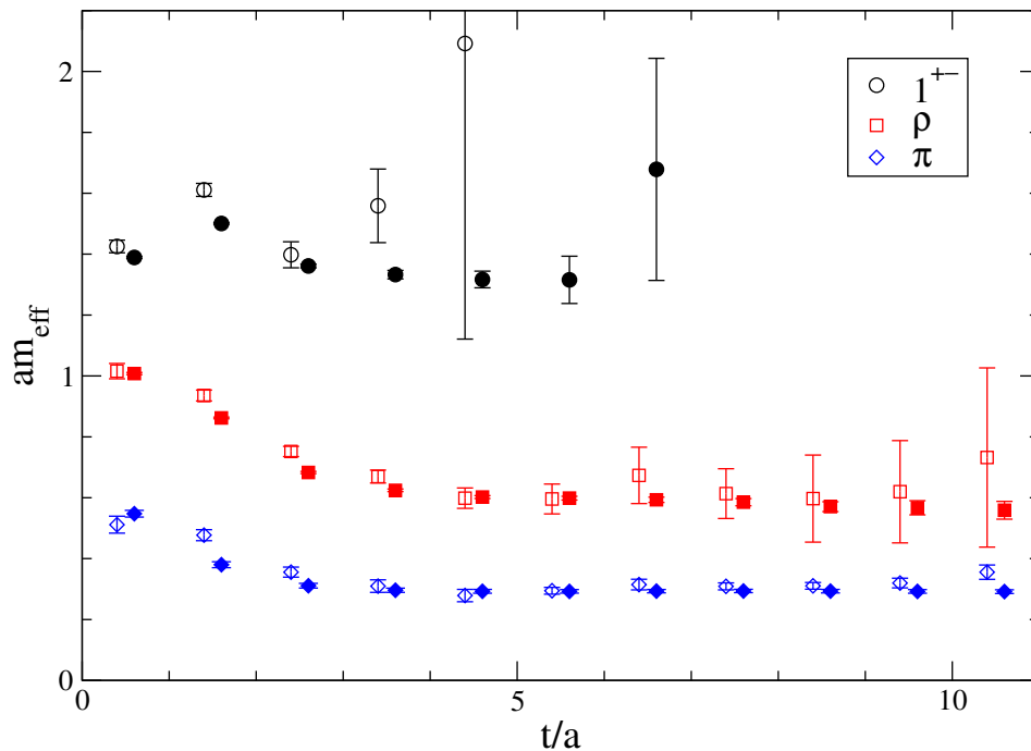
Fig. 5. Comparison of spectrum from all-to-all and point-to-all propagators. The open symbols are point-to-all, the closed symbols all-to-all with 100 eigenvectors and time, colour, spin and space-even-odd dilution.
