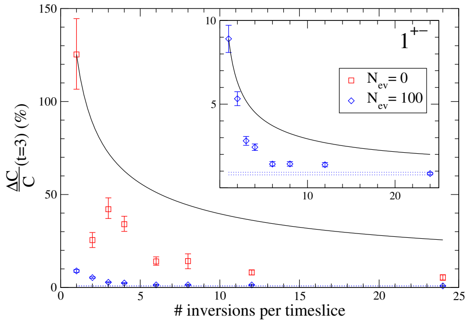
Fig. 8. As Fig. 7, for the 1^{+-} P-wave.
