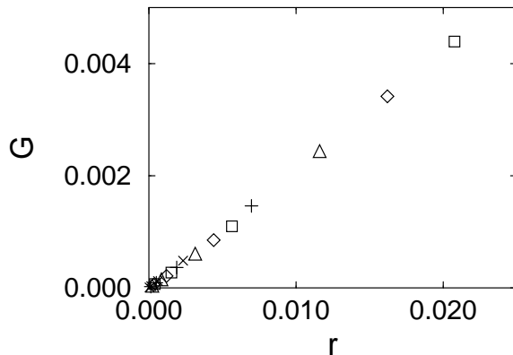
Figure 3. 2D XY model (Lee-Yang case).
