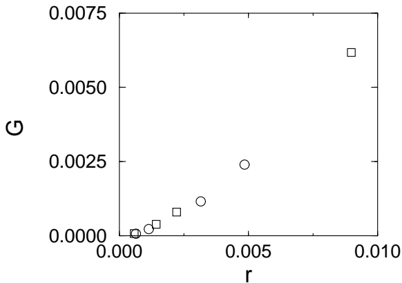
Figure 2. 4D Abelian surface gauge model.
