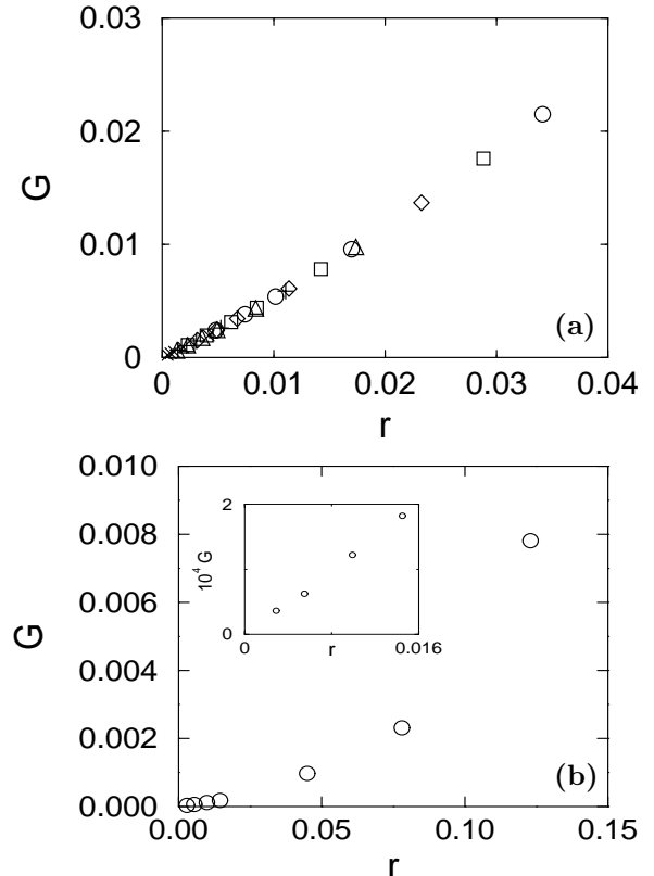
Figure 1. Distribution of partition function zeroes. (a) 2D 10-state Potts model and (b) 3D L_t = 4 SU(3) lattice gauge theory.
