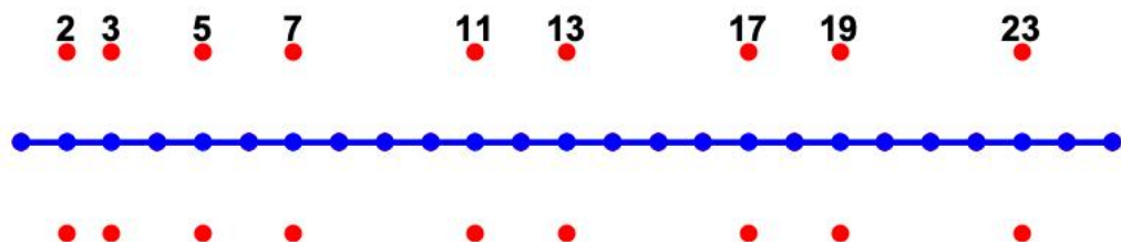
FIGURE 1. The natural numbers from 1 to 25, with the first nine primes plotted (in red) at equal distances above and below.
