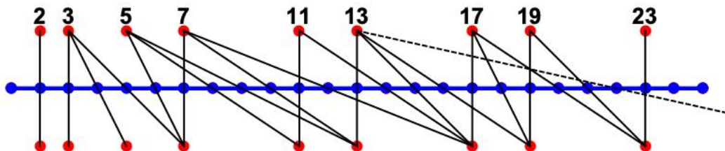
FIGURE 2. The line from p_1 above to p_2 below crosses the number line at the mean value (p_1 + p_2)/2 . There is an intersection of some line of this sort for every n \geq 2 .
