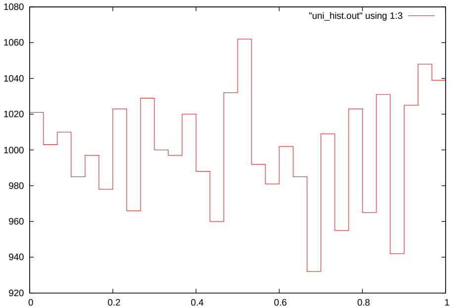
Random numbers per bin, total of 30 bins and 30000 numbers
