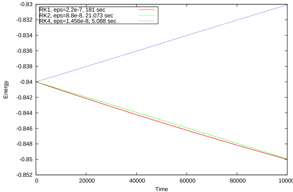
Adaptive methods for Kepler problem
