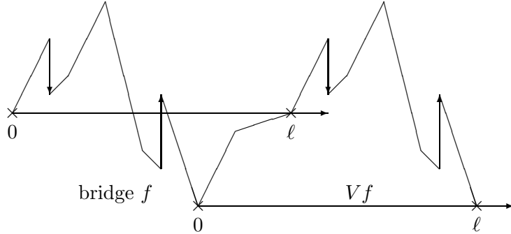
Figure 1: A càdlàg bridge and its Vervaat's transform
