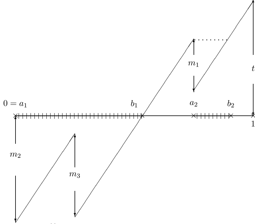
Figure 2: \varepsilon_{\mathbf{m}}^{(t)} and intervals of constancy of its supremum.
