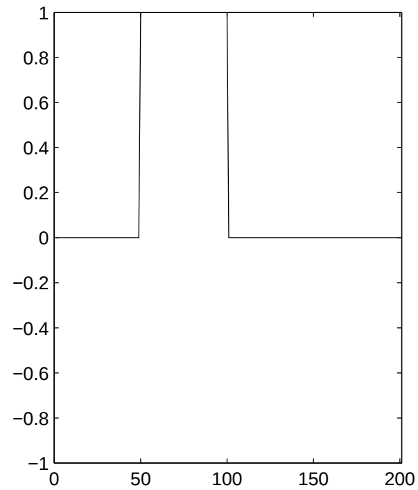
Initial data u_0
