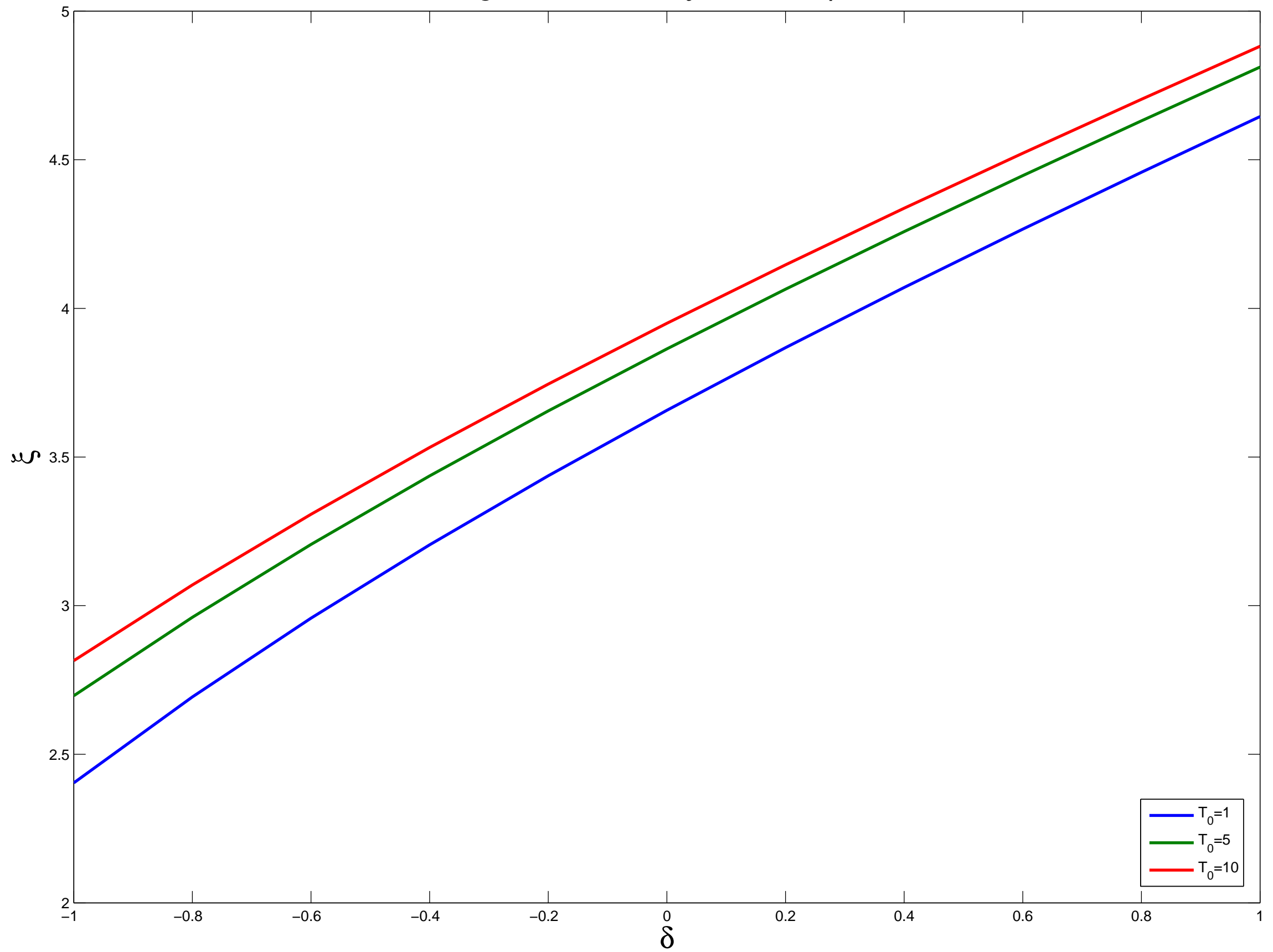
Fig2: Variation of \xi with \delta for \beta=0
