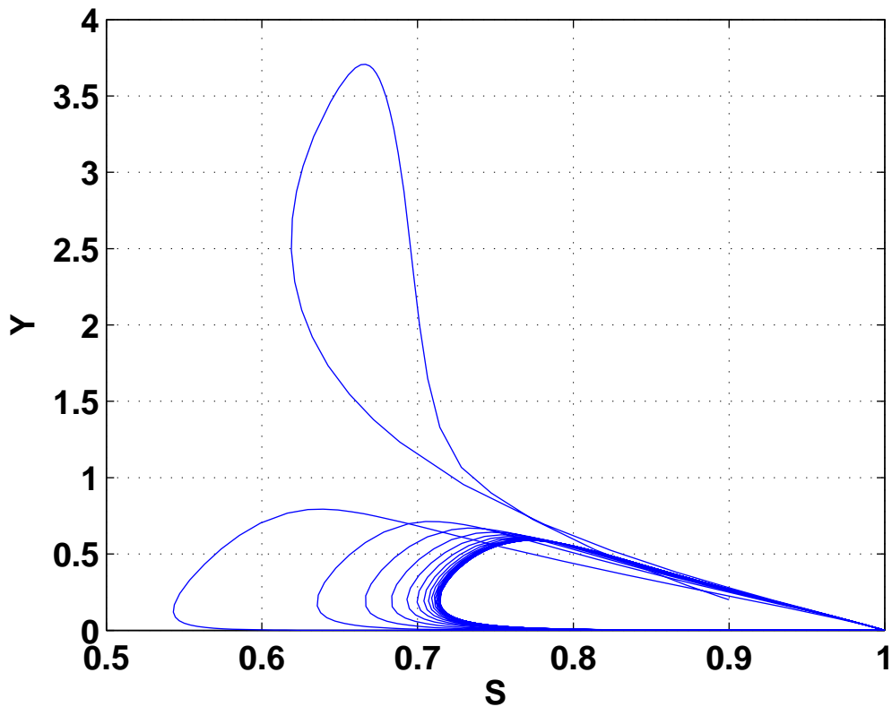
Phase plane plot of prey (S) and predator (Y)
