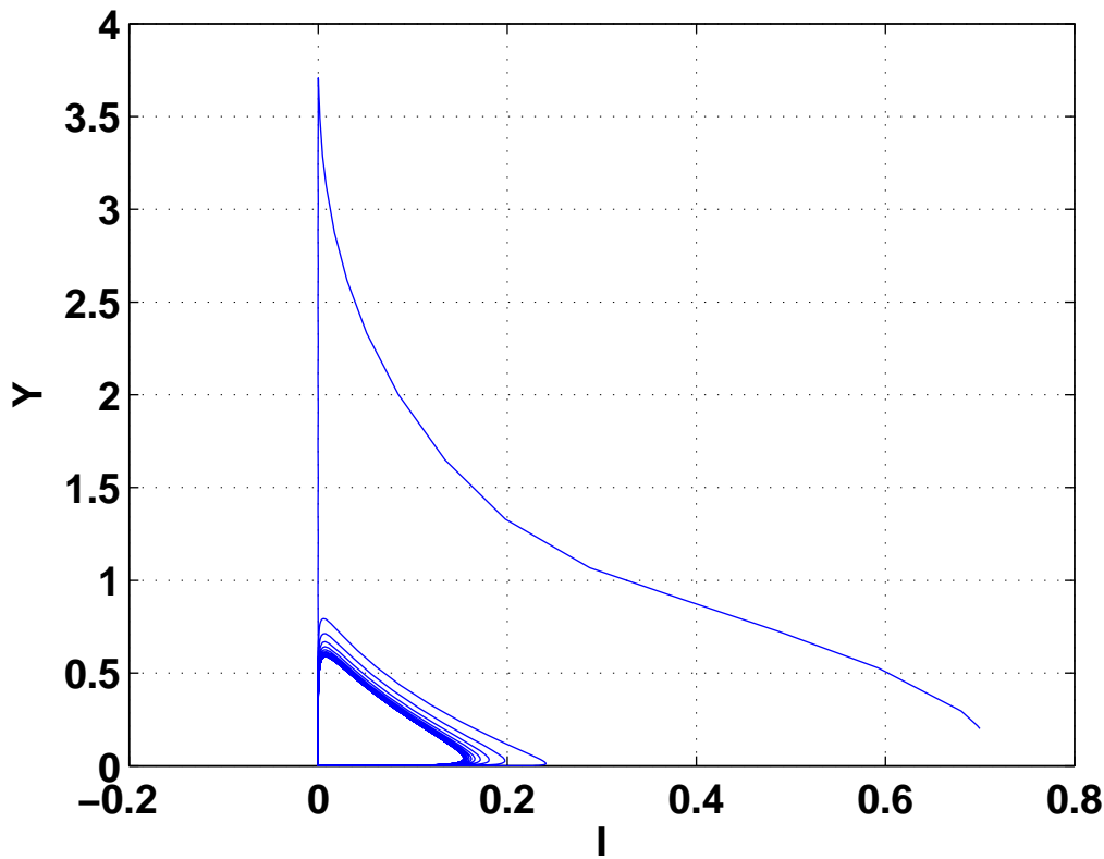
Phase plane plot of infected prey ( I ) and predator ( Y )
