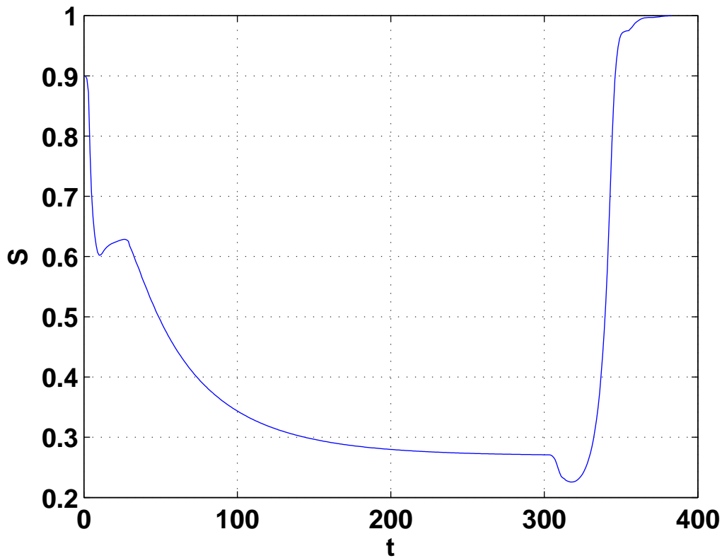
Variation of healthy prey population with time
