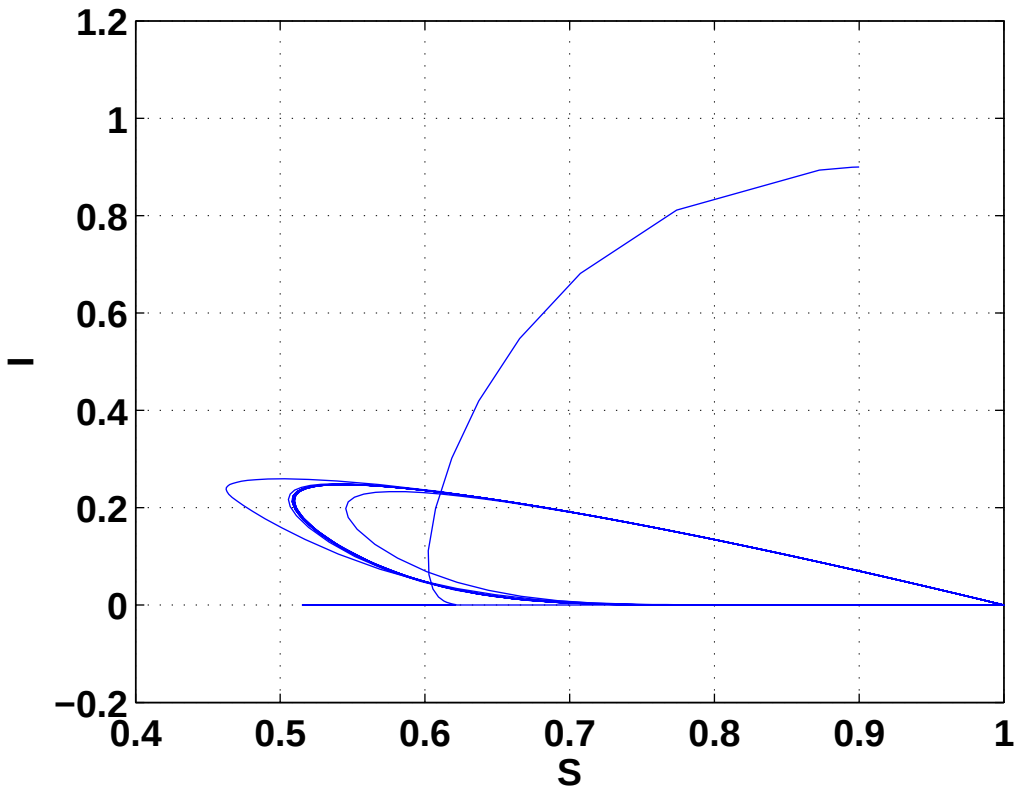
Phase plane plot of susceptible prey ( S ) and infected prey ( I )
