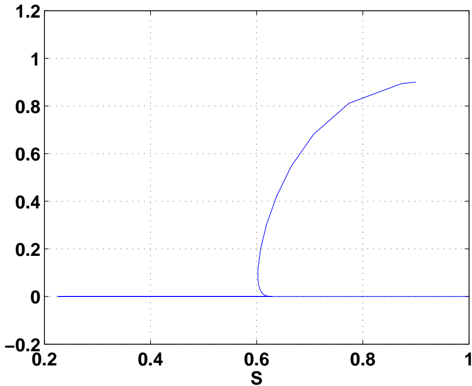
Phase plane plot of susceptible prey ( S ) and infected prey ( I )
