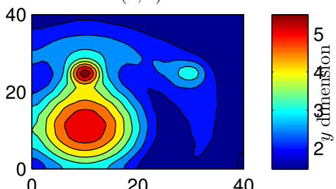
w(x, 1).
