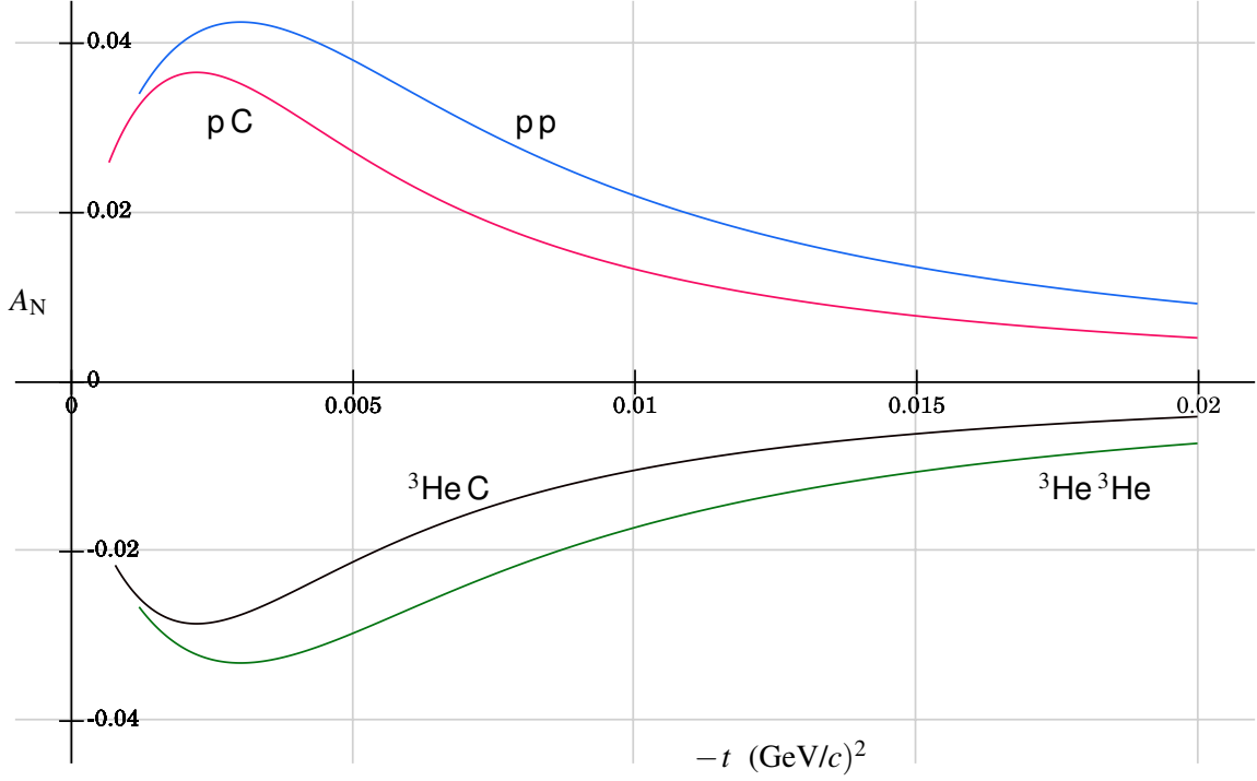
Figure 1: Analyzing power A_N versus the squared momentum transfer variable (-t) for the elastic scattering processes (from the top): (1) proton proton, (2) proton carbon, (3) helium-3 carbon, (4) helium-3 helium-3, assuming that \sigma_{\text{tot}}(\text{hC}) = 2\sigma_{\text{tot}}(\text{pC}) , that \sigma_{\text{tot}}(\text{hh}) = 4\sigma_{\text{tot}}(\text{pp}) , and that \rho , \delta , R_S , I_S , and finite nuclear size effects are negligible.
