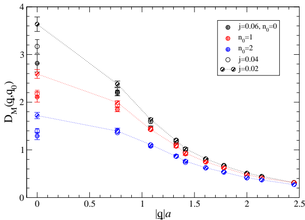
Fig. 18. Magnetic gluon propagator at \mu = 0.7 for various values of the diquark source j .
