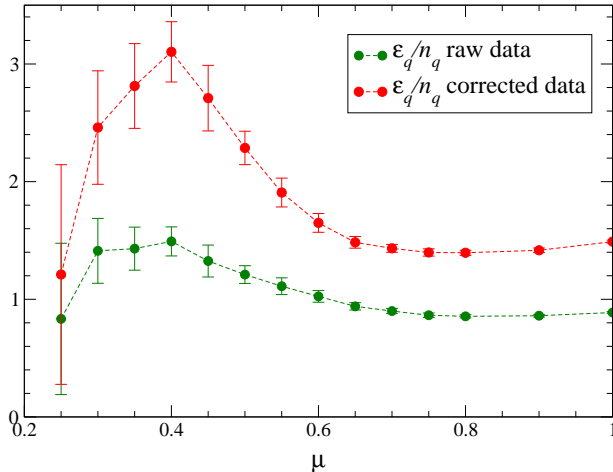
Fig. 19. The ratio \varepsilon_q/n_q vs. \mu , using both the raw data of table 4, and rescaled by a factor n_{SB}^{\text{lat}}/\varepsilon_{SB}^{\text{lat}}
