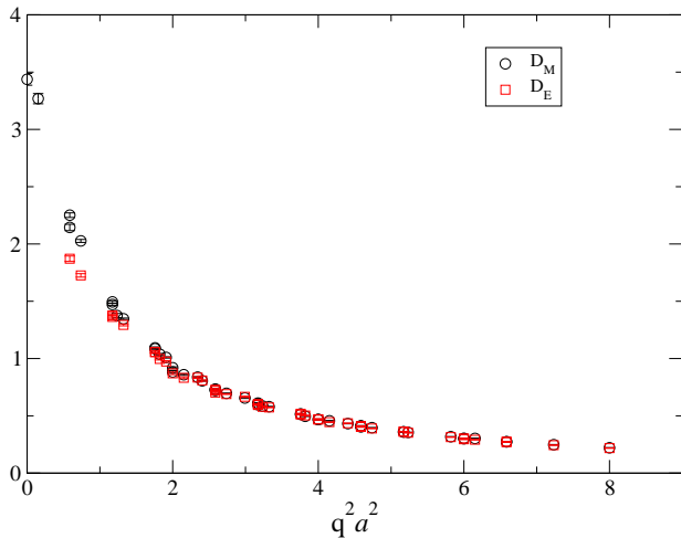
Fig. 14. Gluon propagator at \mu = j = 0 .
