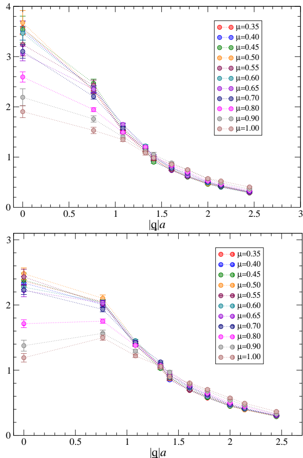
Fig. 16. Magnetic gluon propagator for q_0 = 0 (top) and aq_0 = 2 \sin \pi/16 (bottom) and diquark source j = 0.04 , as a function of spatial momentum |\mathbf{q}| for various values of the chemical potential.
