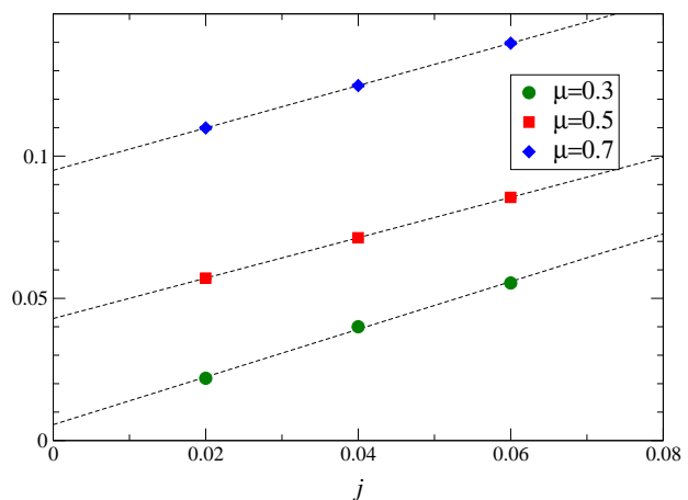
Fig. 10. Superfluid condensate \langle qq \rangle vs. j for various \mu
