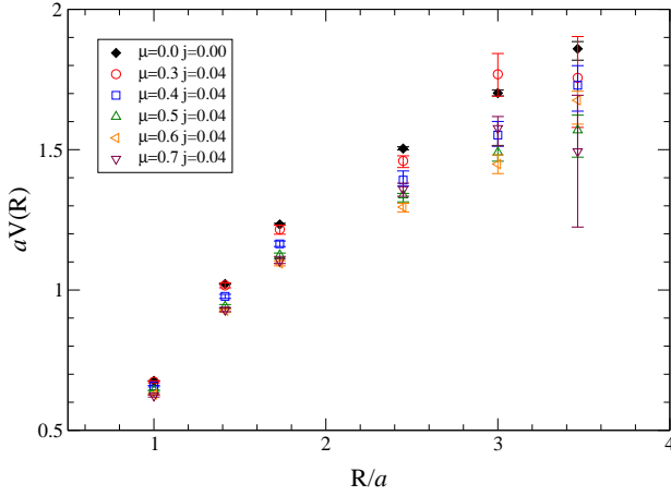
Fig. 11. The static quark potential for various values of the chemical potential \mu and diquark source j = 0.04 , together with the \mu = j = 0 potential shown in fig. 2.
