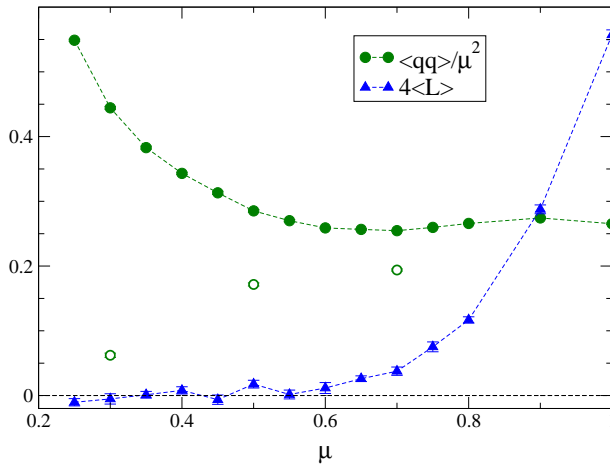
Fig. 9. The Polyakov loop L and the superfluid diquark condensate \langle qq \rangle/\mu^2 for j = 0.04 as function of \mu . Open symbols show \langle qq \rangle/\mu^2 extrapolated to j = 0 .
