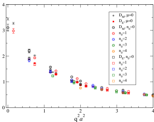
Fig. 15. Gluon propagator at \mu = 0.7, j = 0.04 , together with the \mu = j = 0 propagator for comparison.
