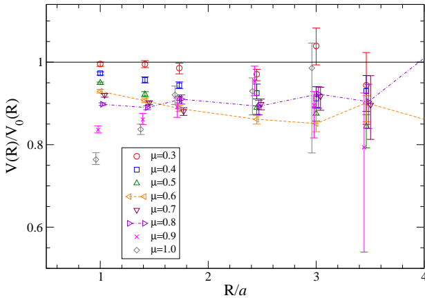
Fig. 12. The static quark potential for various values of the chemical potential \mu and diquark source j = 0.04 , divided the \mu = j = 0 potential shown in fig. 2.
