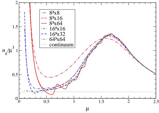
Fig. 4. n_{SB}^{\text{lat}}/\mu^3 for free massless Wilson fermions.
