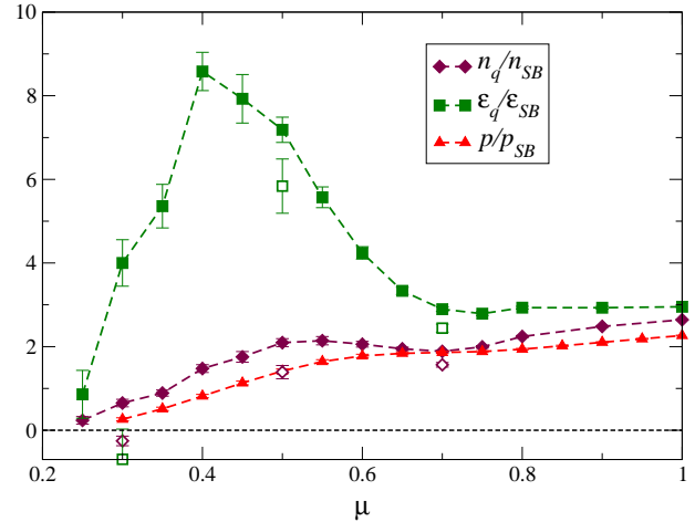
Fig. 5. Ratio of thermodynamic observables to free field values versus \mu for j = 0.04 . Open symbols show extrapolations to j = 0 .
