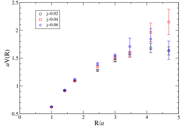
Fig. 13. The static quark potential at \mu = 0.7 for different values of j .
