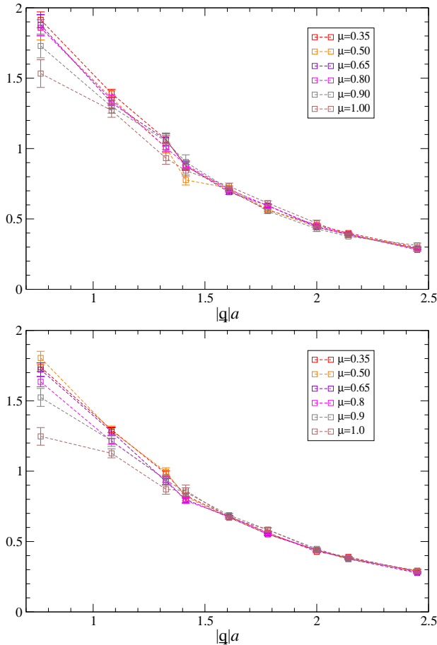
Fig. 17. As fig. 16, for the electric gluon propagator.
